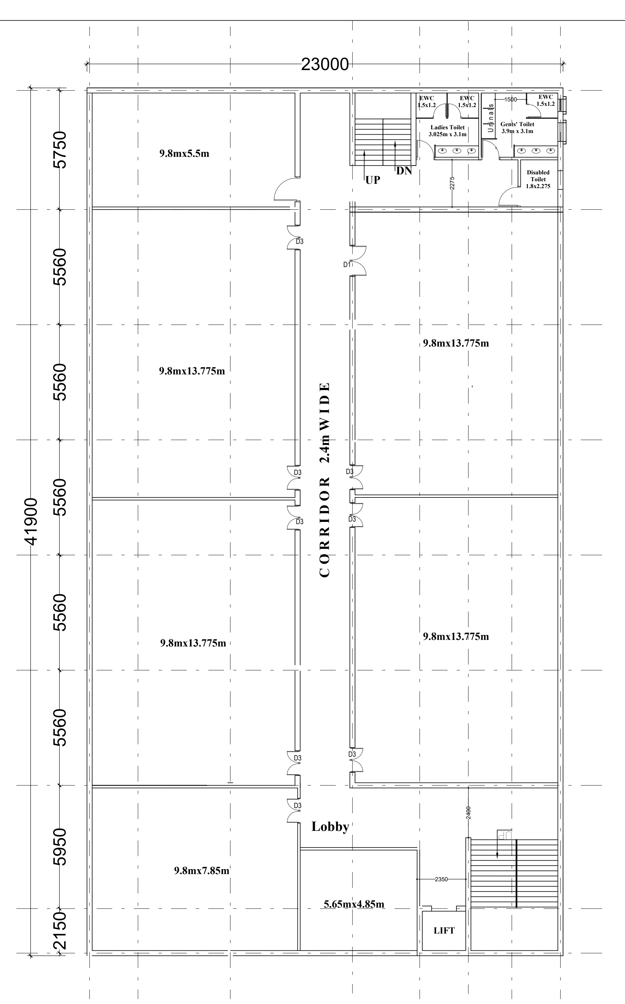
2nd Floor Plan (may be allocated to Chemistry dept.)
