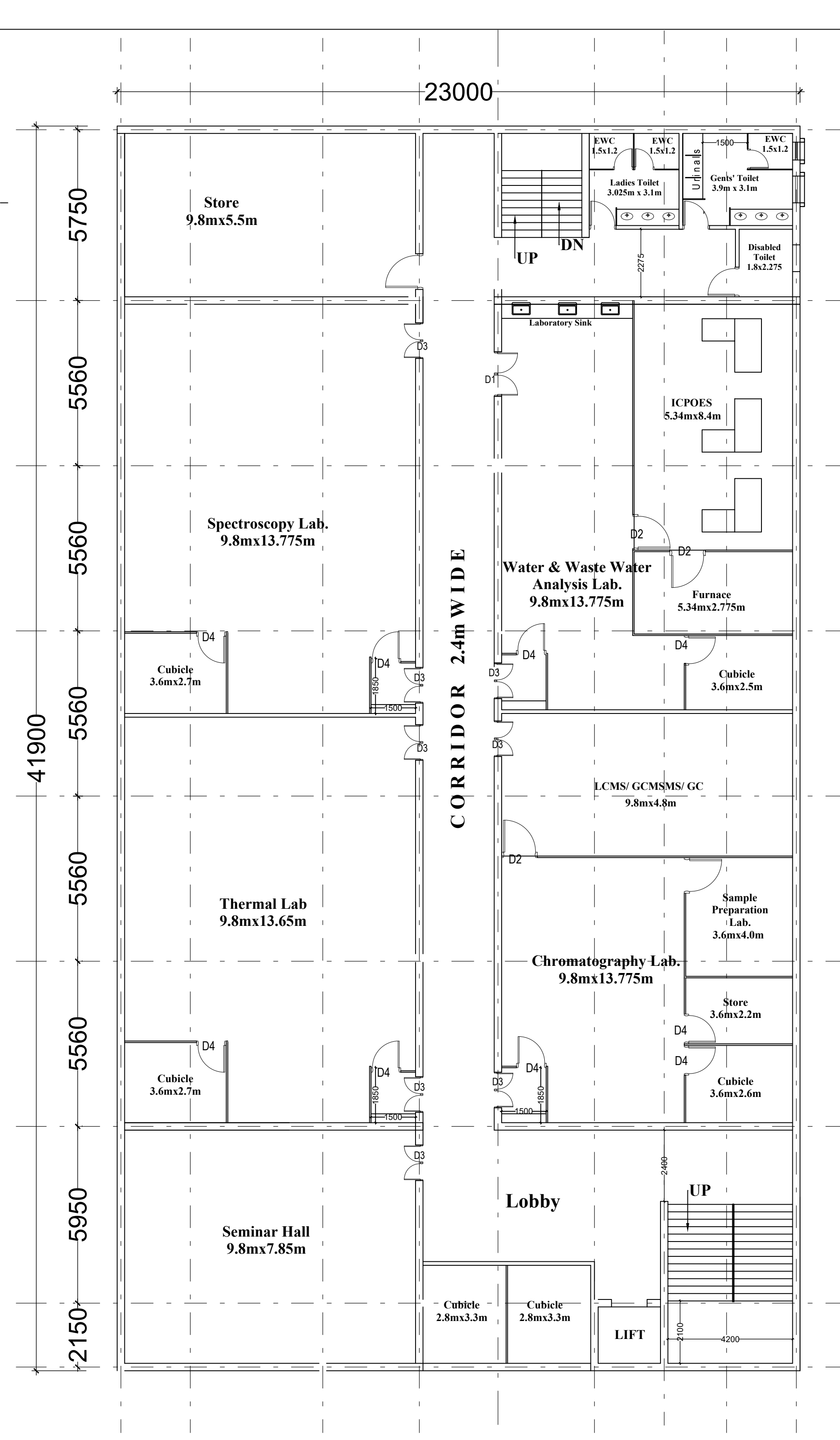
1st Floor Plan
