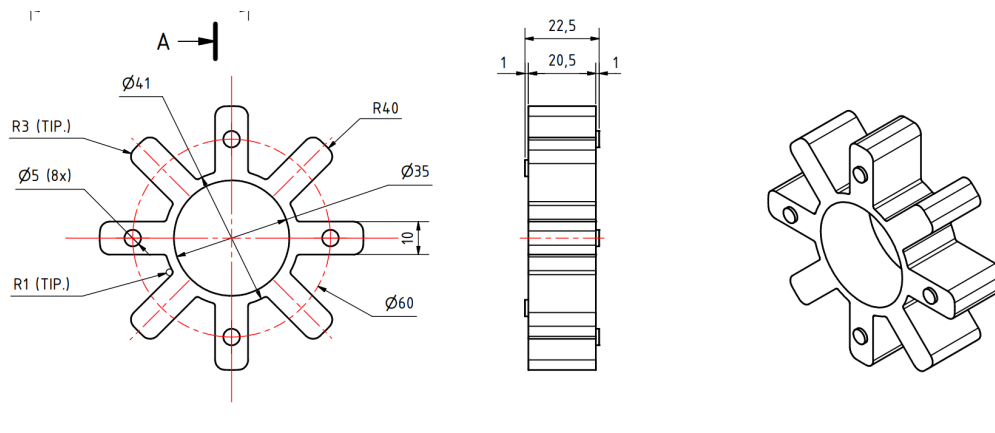
Fig 2:- Drawings of the Part discussed with attendees.
