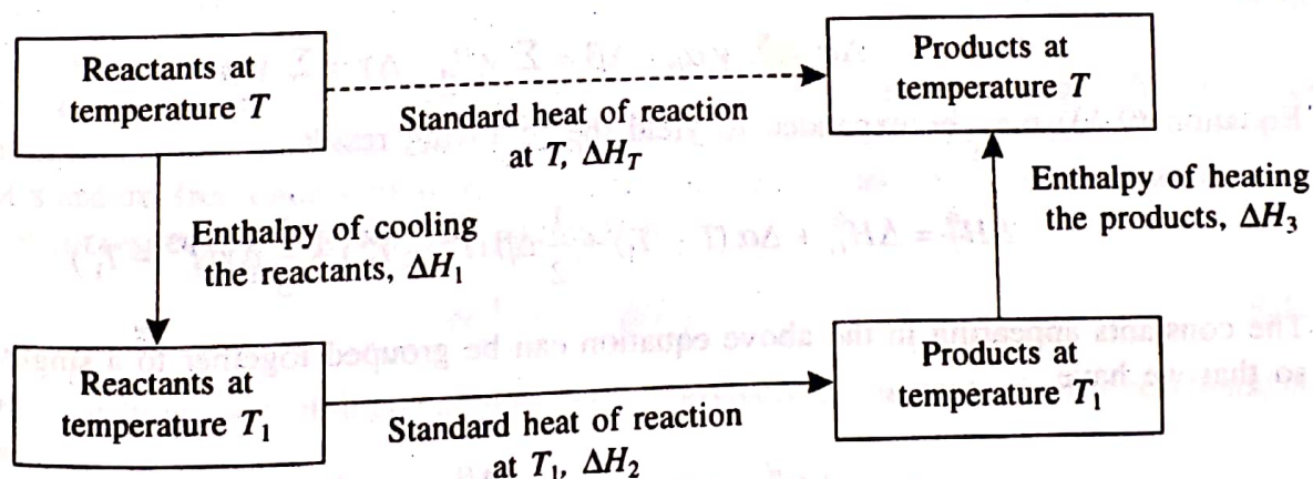
Fig. 9.3 Method of estimating the standard heat of reaction at temperature T given the standard heat of reaction at T_1 .
