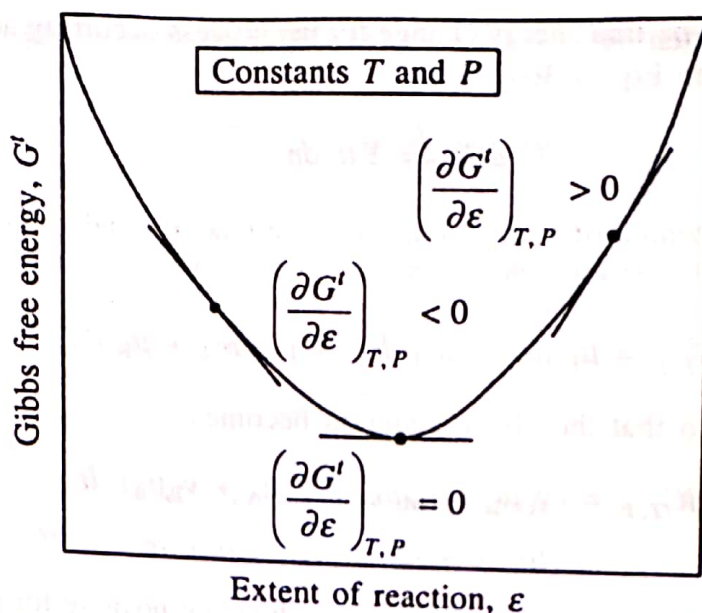
Fig. 9.1 Gibbs free energy of the reaction mixture versus extent of reaction.
