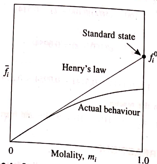
Fig. 9.4 Standard state based on Henry's law.
